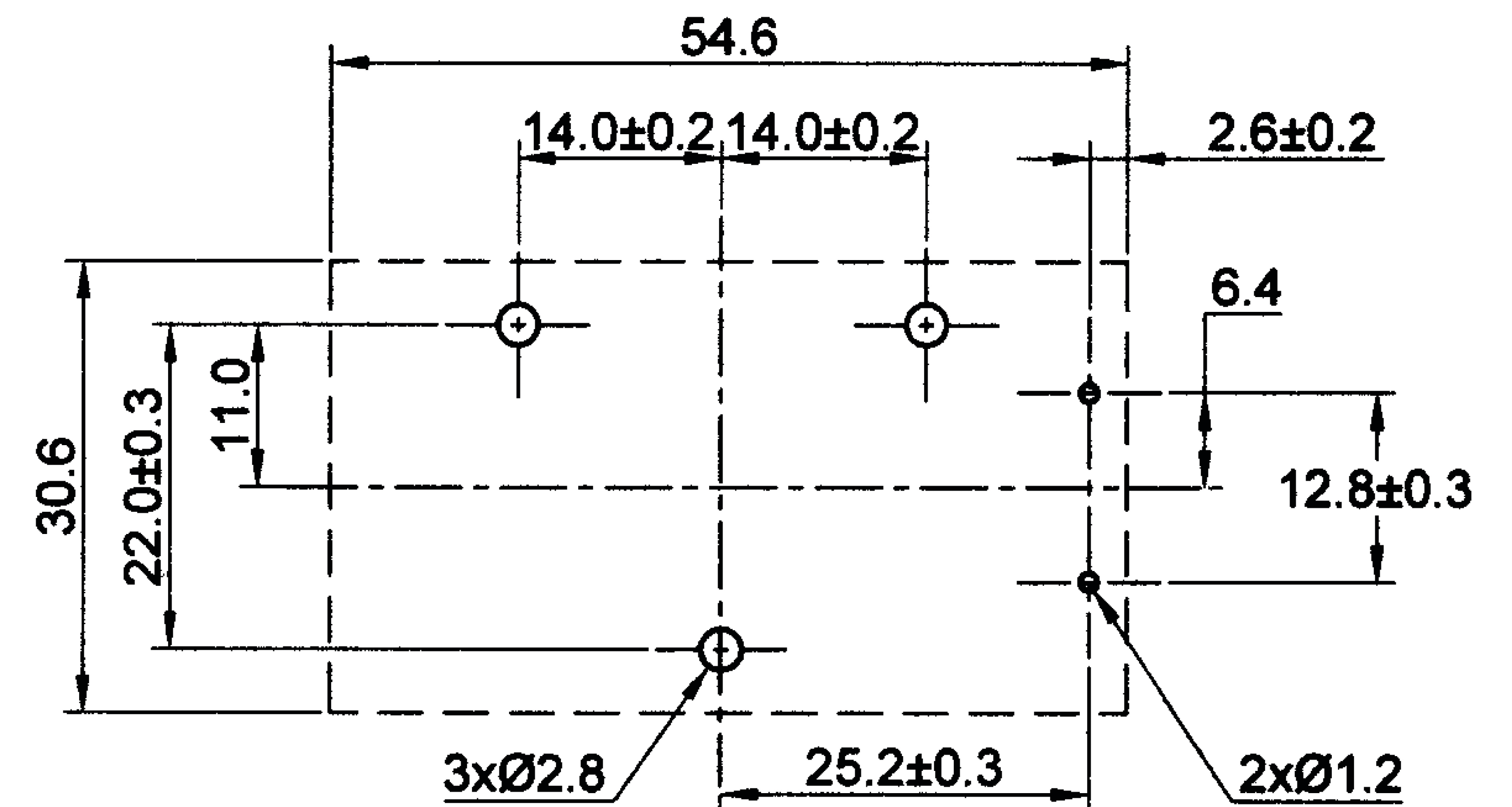
PCB/MOUNTING LAYOUT
